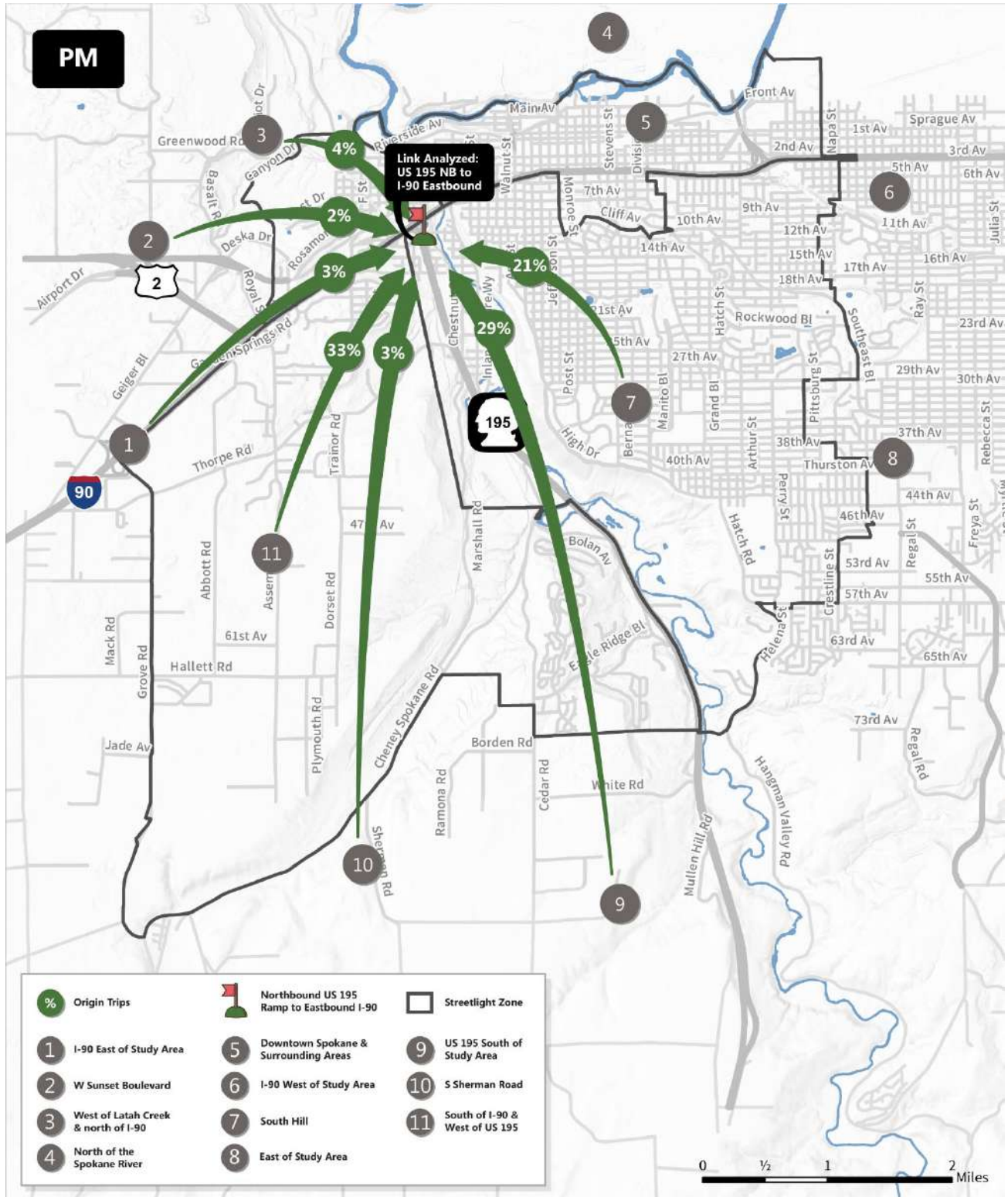
Figure 6. PM Peak Hour US 195 Northbound to I-90 Eastbound Origins
