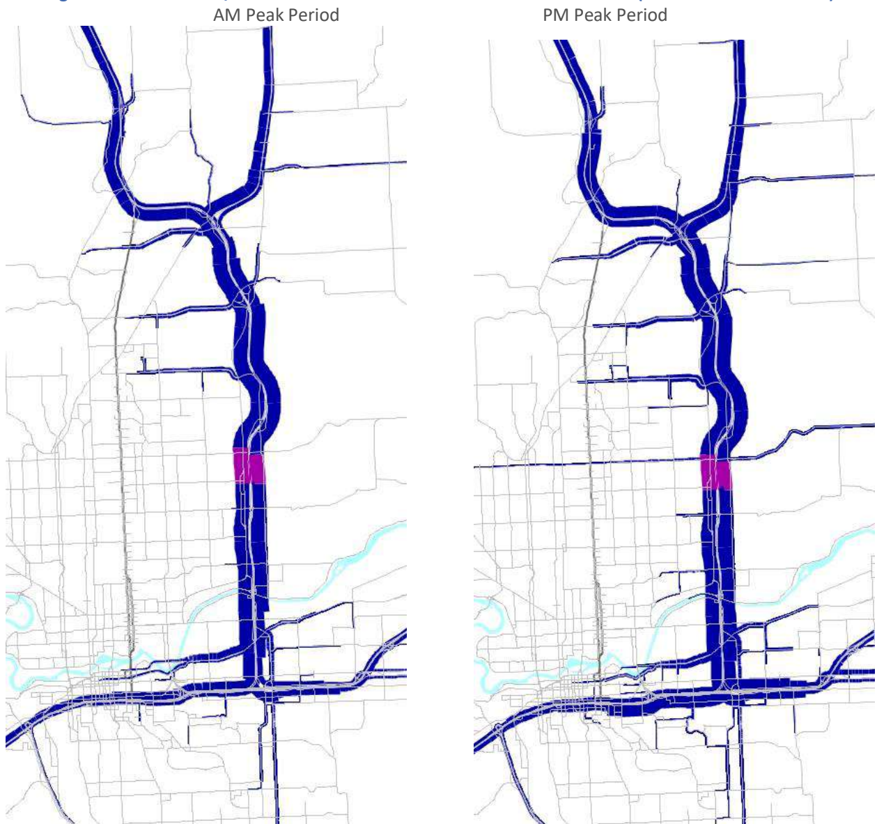
Figure 10: No Build AM/PM Peak Period Flow Bundle - North-South Corridor (South of Francis Avenue)
