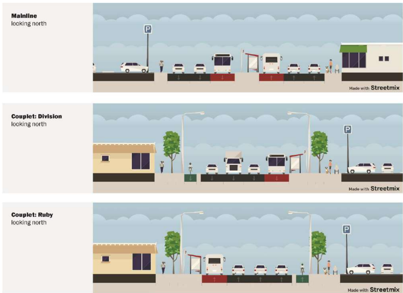
Figure 11. Scenario Center Running Cross Section
