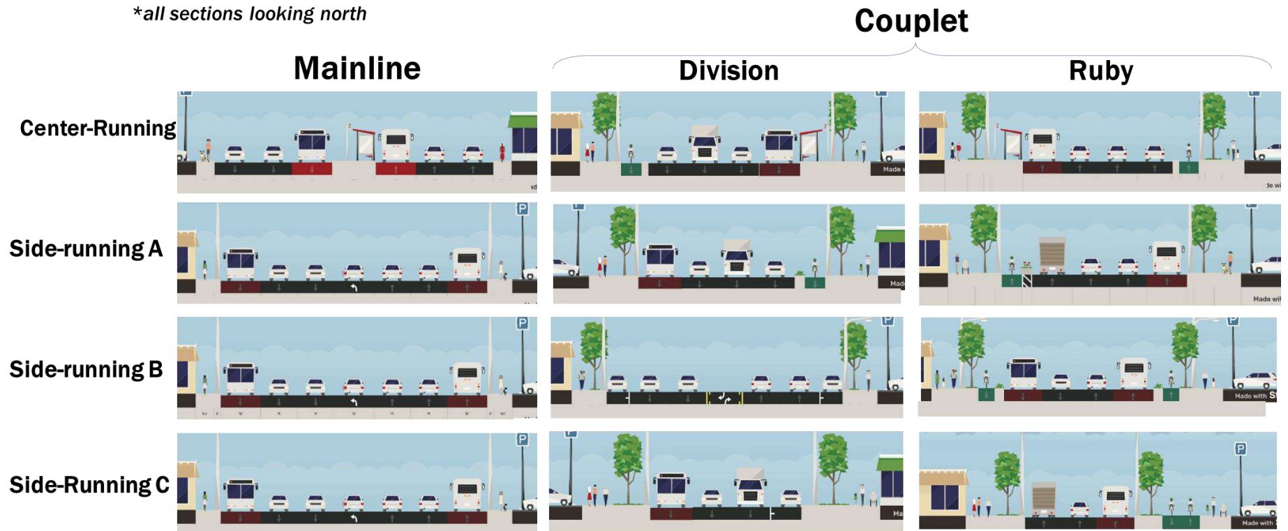
Figure 2: Alternative Roadway Configurations
